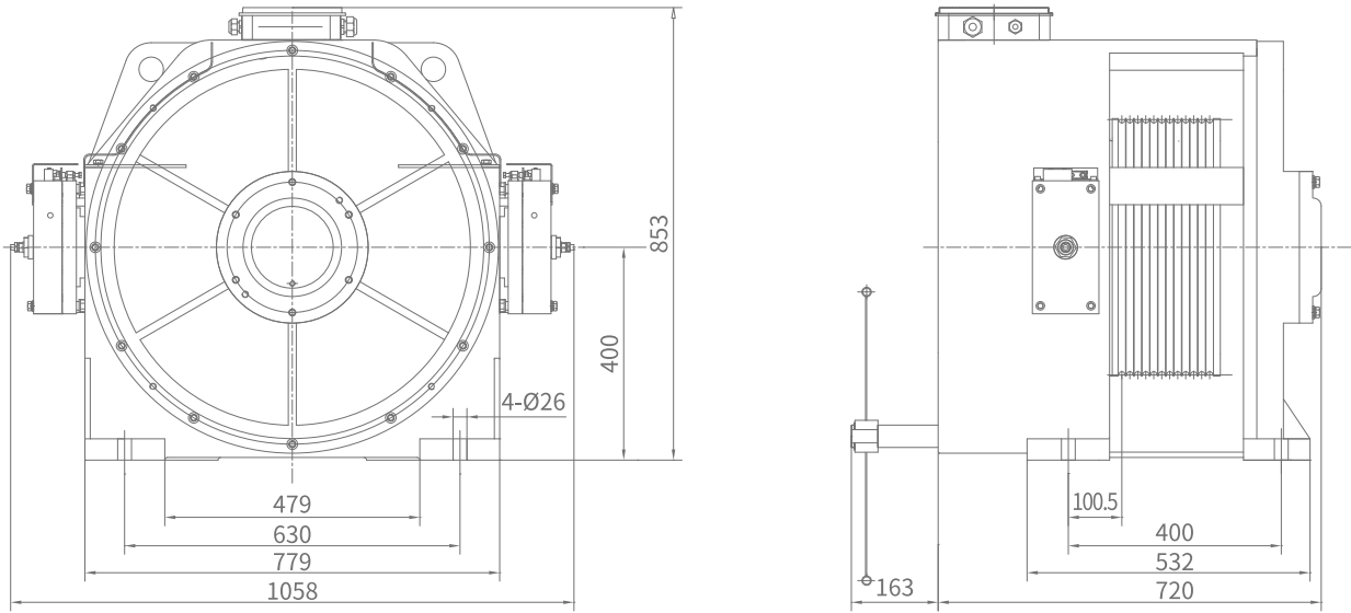
Outline drawing
