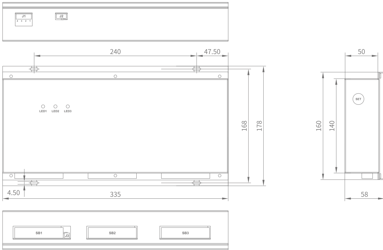
Outline drawing
