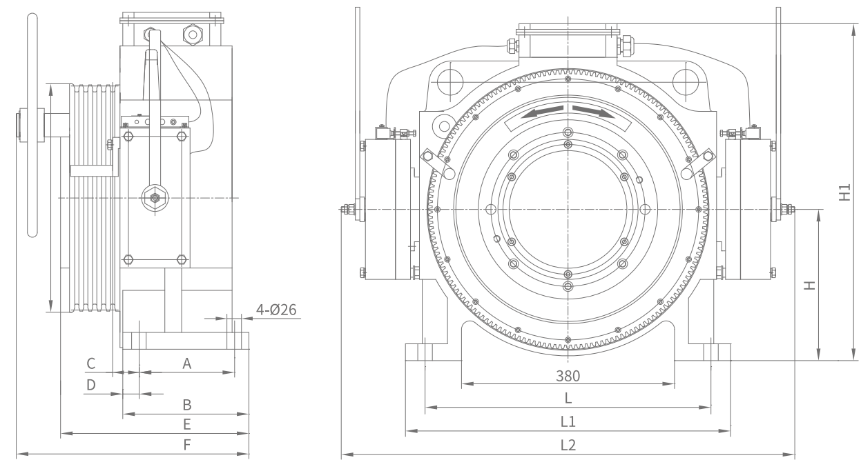
Outline drawing
