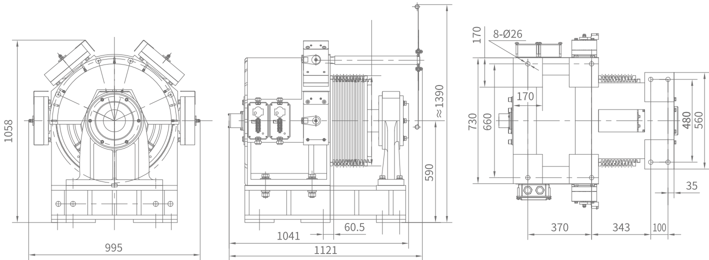
Outline drawing
