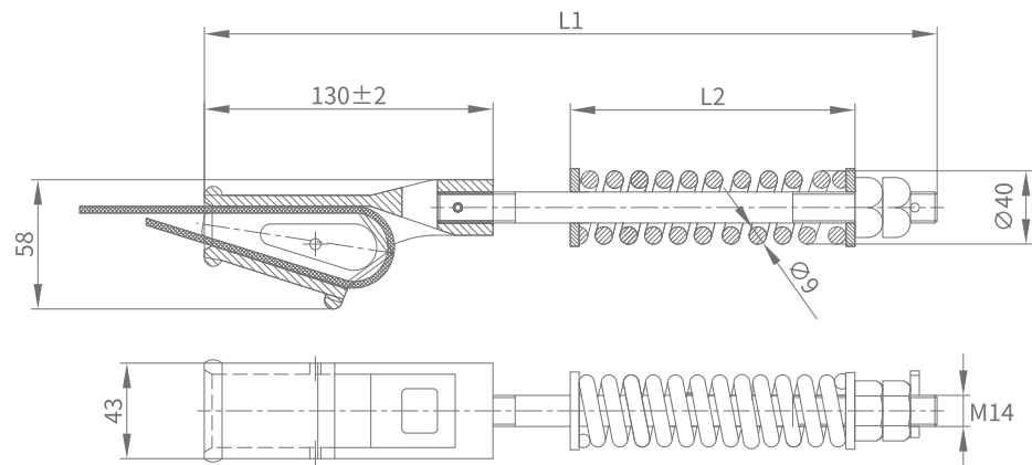
Outline drawing
