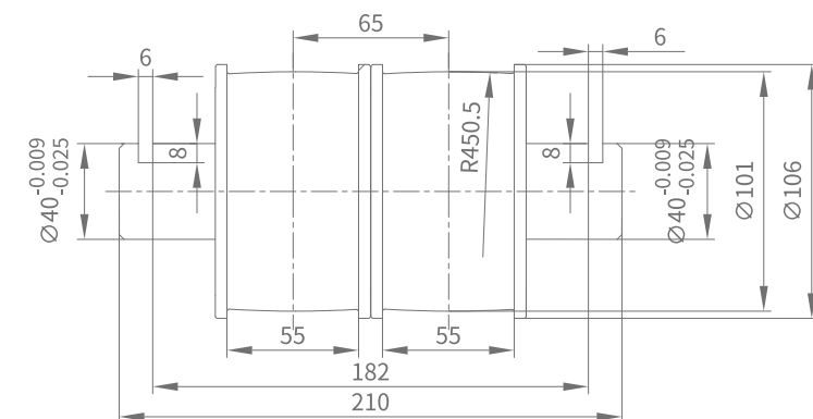
Outline drawing
