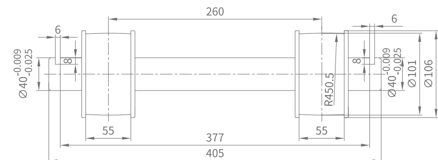
Outline drawing
