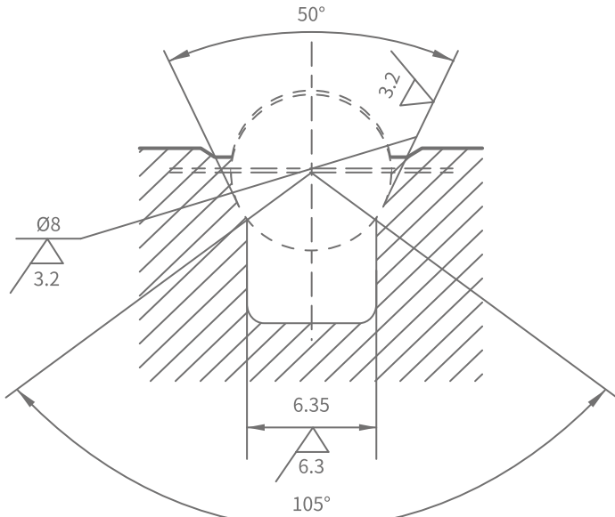
Outline drawing
