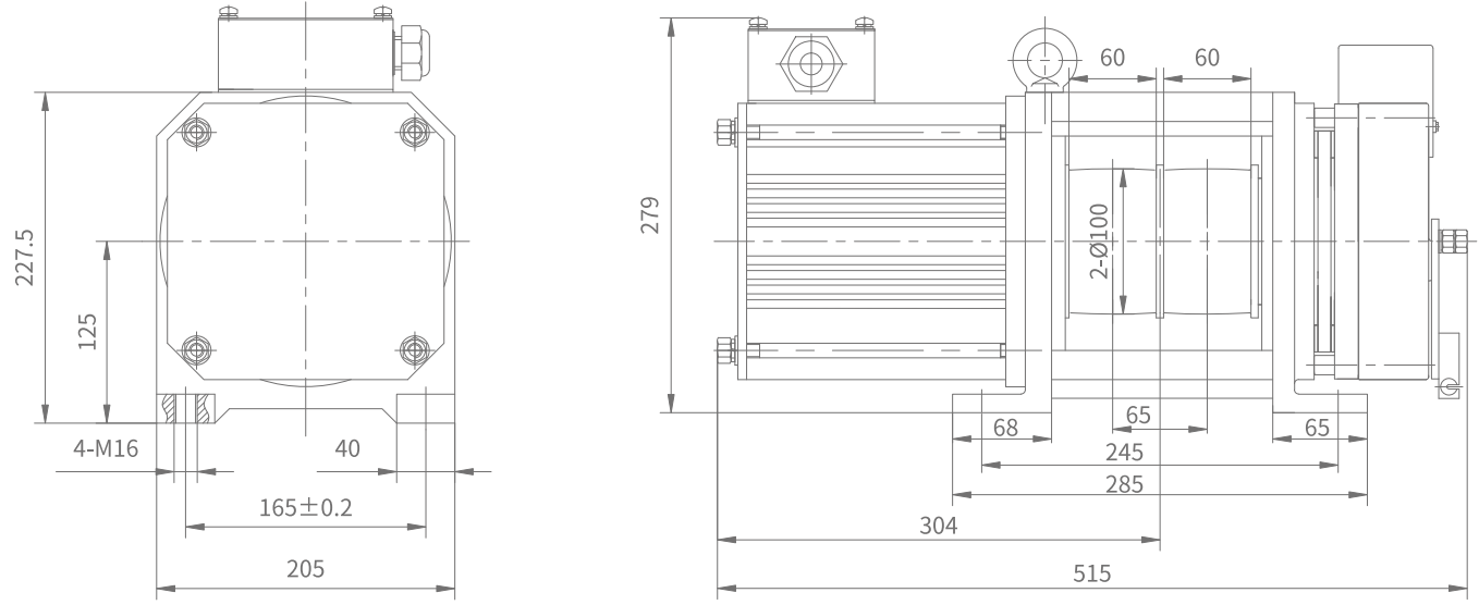
Outline drawing
