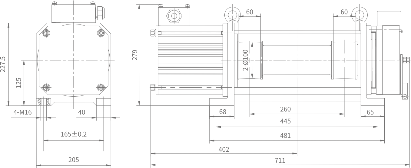
Outline drawing
